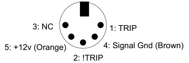
5 Pin DIN Female Connector
