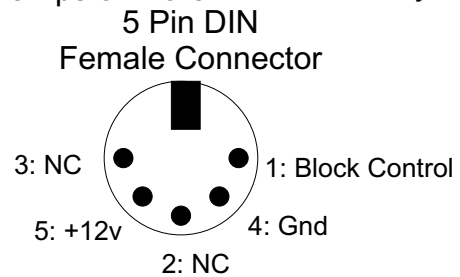
Rayex LM2-12D Relay
