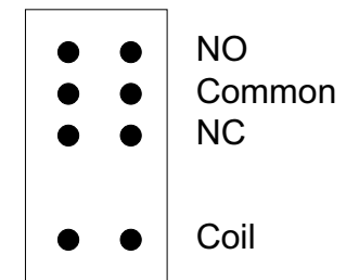
Rayex LM2-12D Relay
